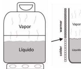
Figure 66 - Example of level measurement through temperature difference.
